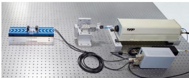
Figure 1 Setup for measurements using external measuring equipment: positioning axis with mount for a reflector mirror, interferometer setup to measure the position
